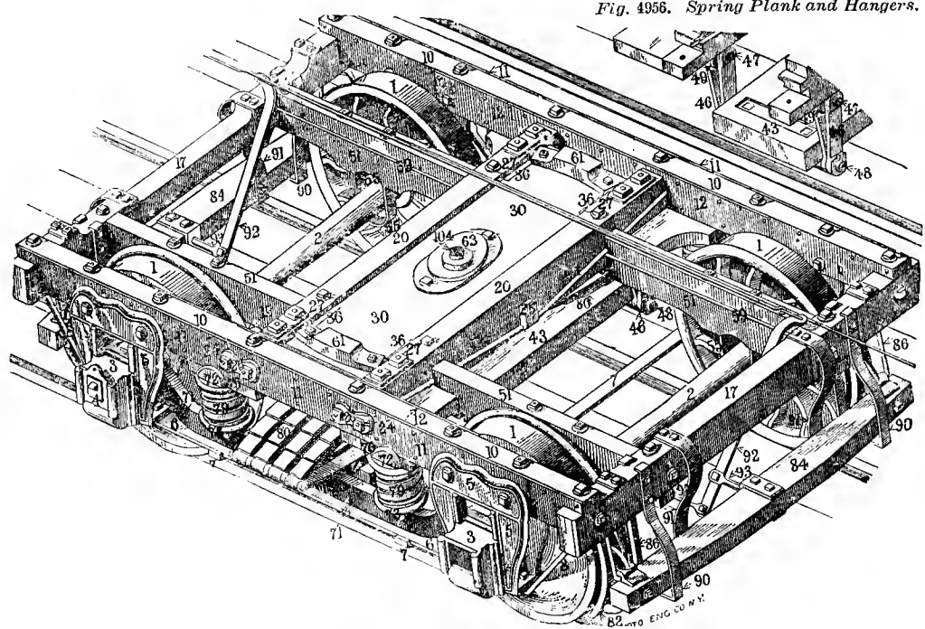
Fig. 4955. A PERSPECTIVE VIEW OF A FOUR-WHEELED TRUCK.
